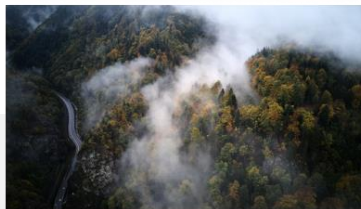
Atmospheric aerosol loading
